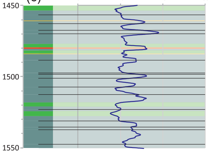
(c) Gamma (API)
