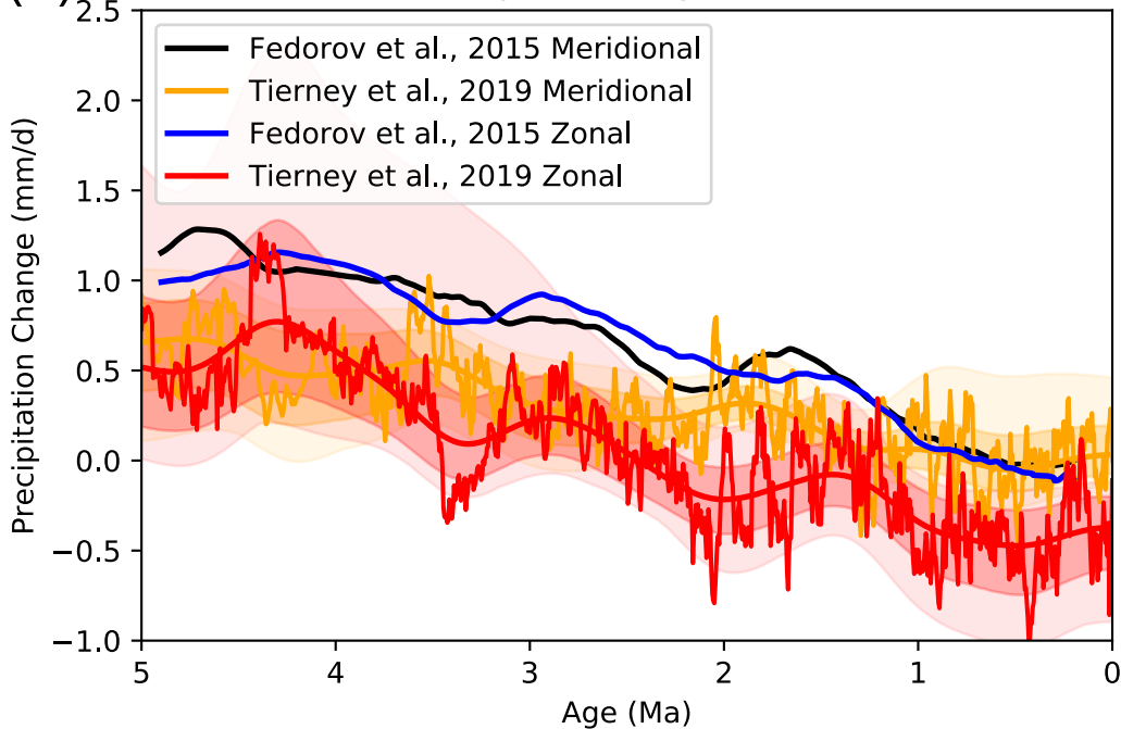
(b) Southwest Precipitation (Synthetic Time Series)
