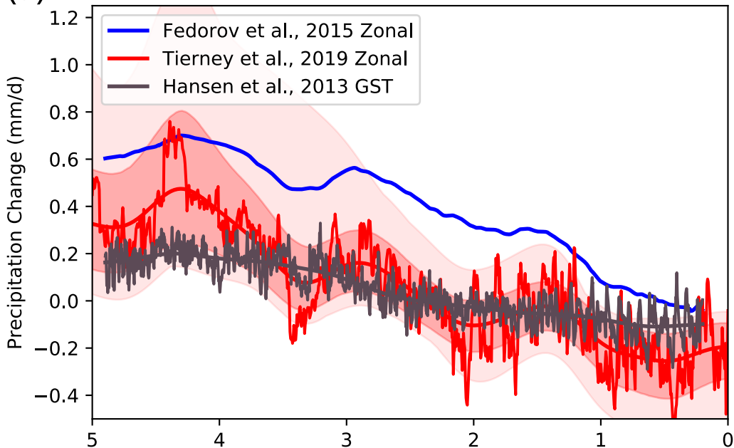
(b) Southwest Precipitation (Synthetic Time Series)
