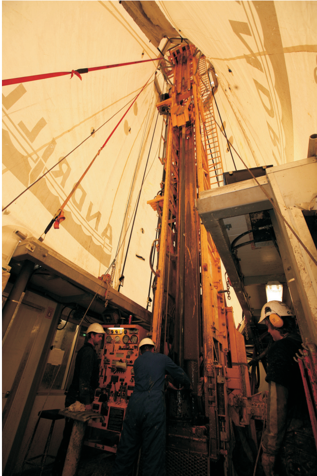
Figure 5. Drilling operations under the ANDRILL drill-rig canopy.
